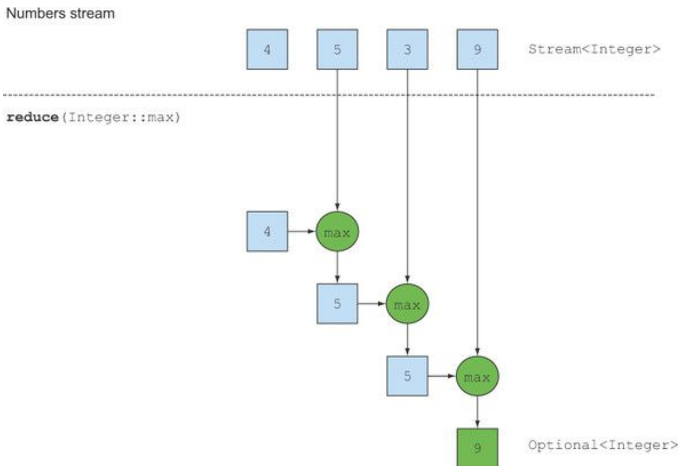
Figure 5.8. A reduce operation—calculating the maximum
