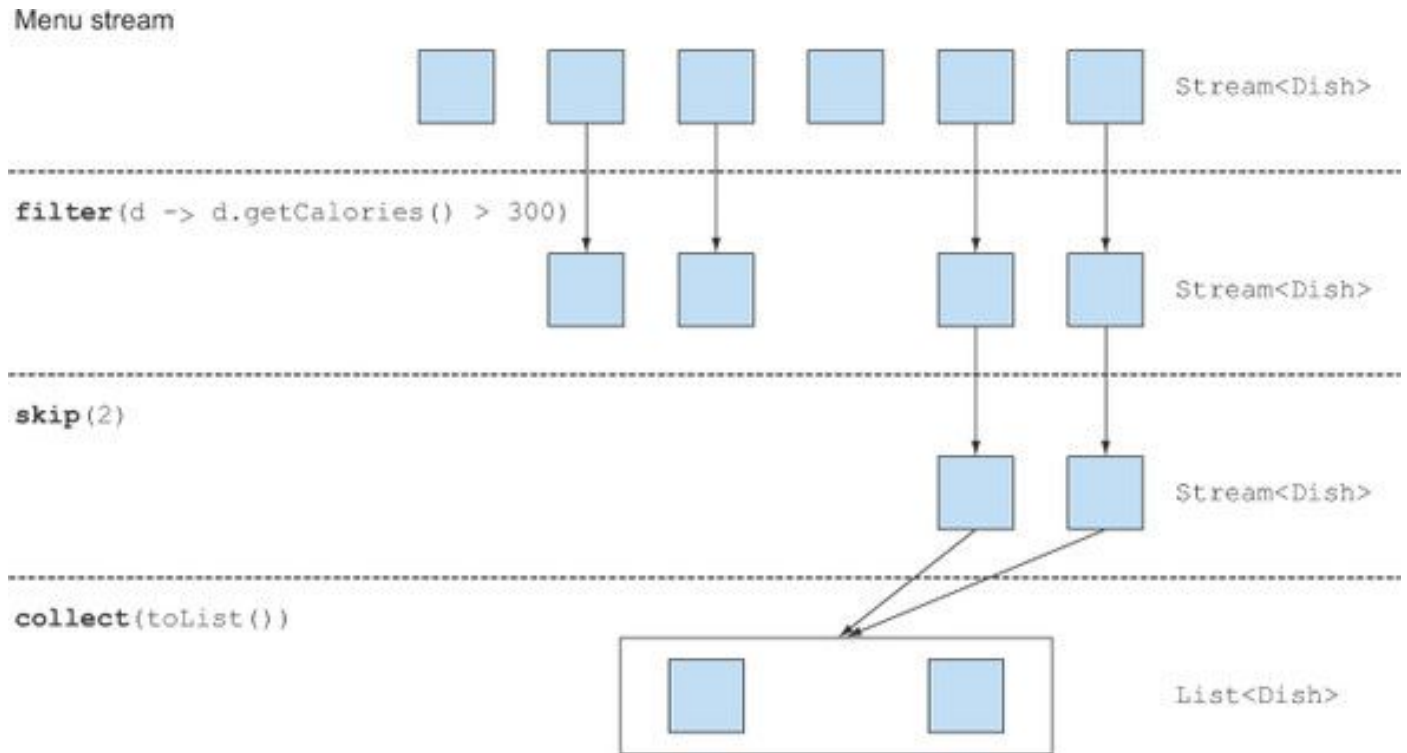
Figure 5.4. Skipping elements in a stream
