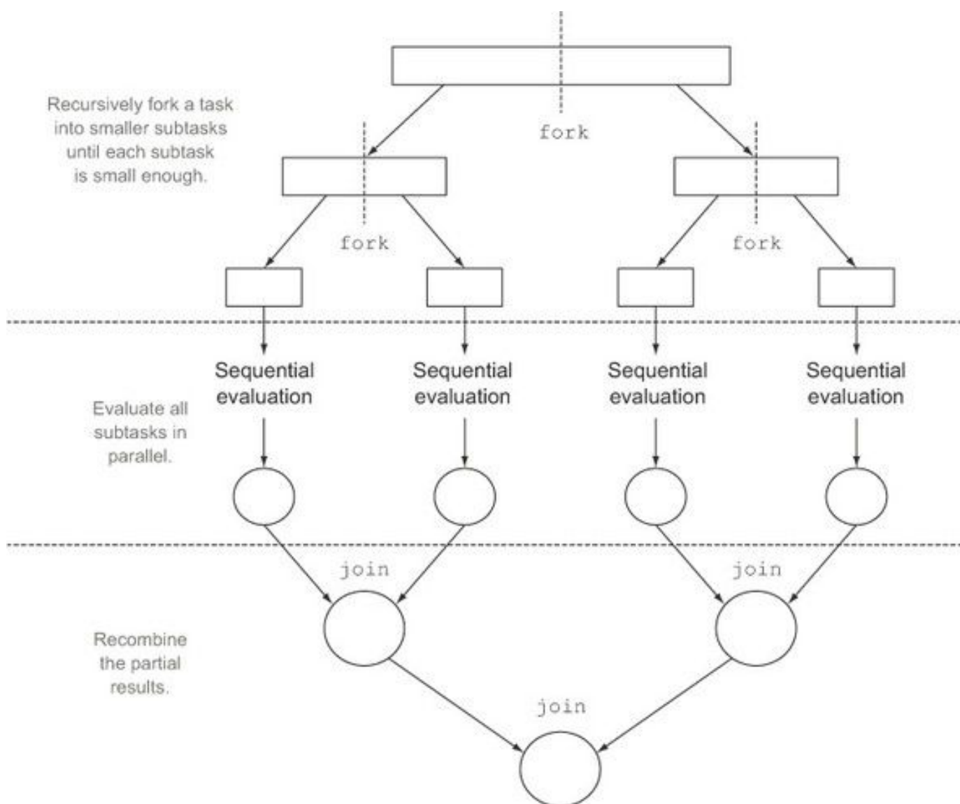
Figure 7.3. The fork/join process
