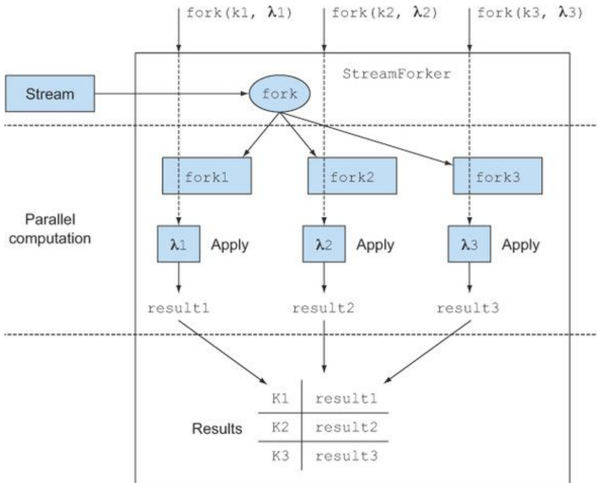
Figure C.1. The StreamForker in action
