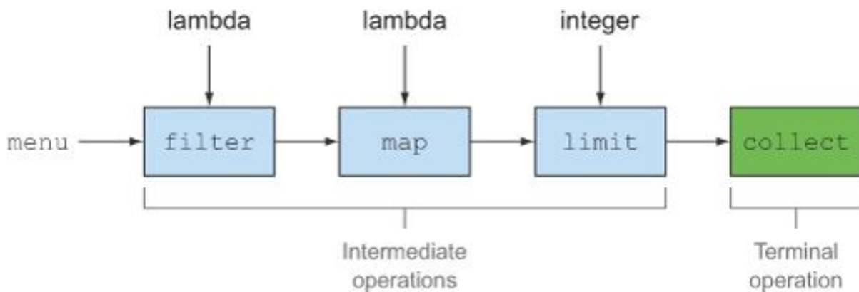
Figure 4.5. Intermediate vs. terminal operations
