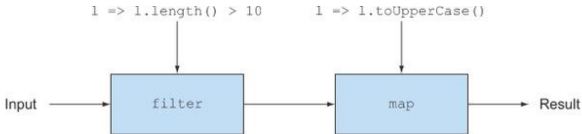
Figure 15.1. Stream-like operations with Scala's List
