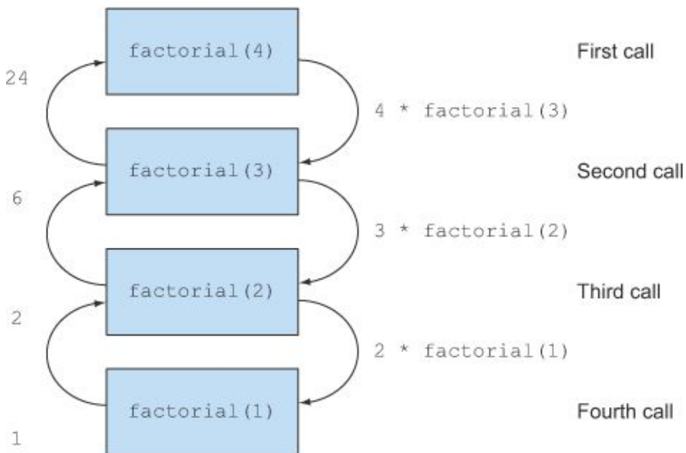
Figure 13.5. Recursive definition of factorial, which requires several stack frames
