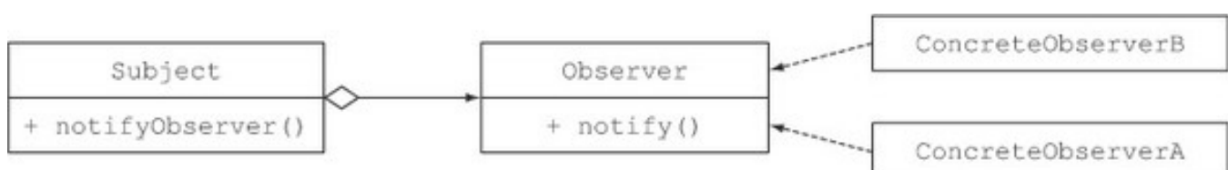
Figure 8.2. The observer design pattern
