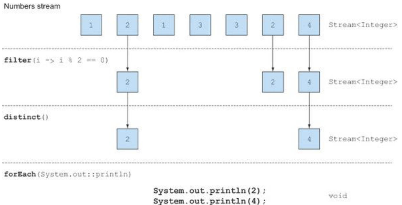
Figure 5.2. Filtering unique elements in a stream
