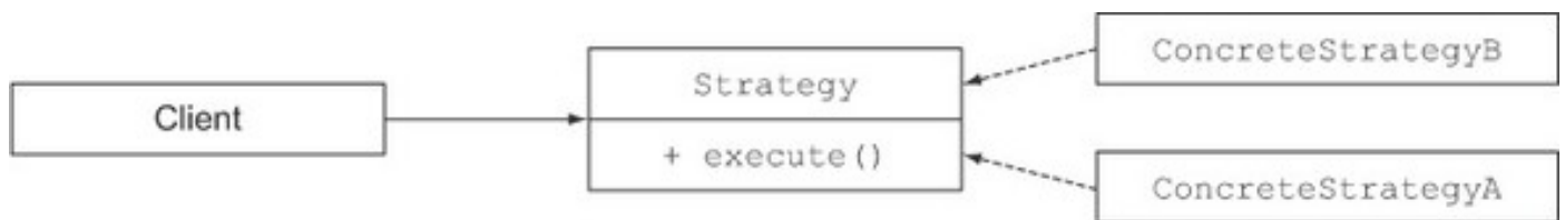
Figure 8.1. The strategy design pattern
