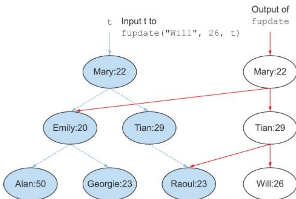
Figure 14.4. No existing data structure was harmed during the making of this update to the Tree.
