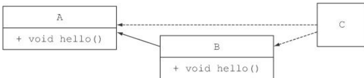
Figure 9.5. The most specific default-providing interface wins.
