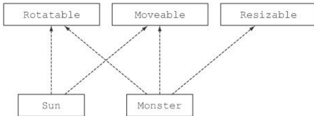
Figure 9.4. Multiple behavior composition
