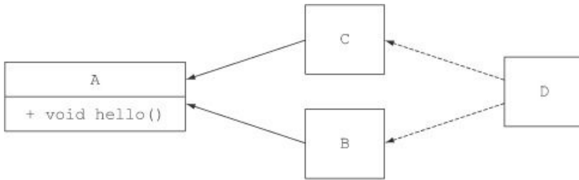
Figure 9.8. The diamond problem
