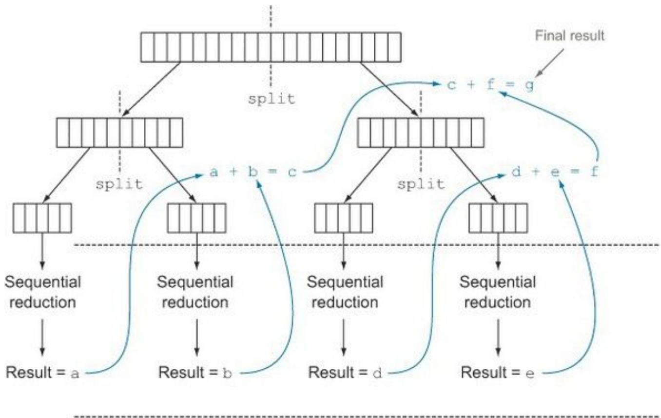
Figure 7.4. The fork/join algorithm
