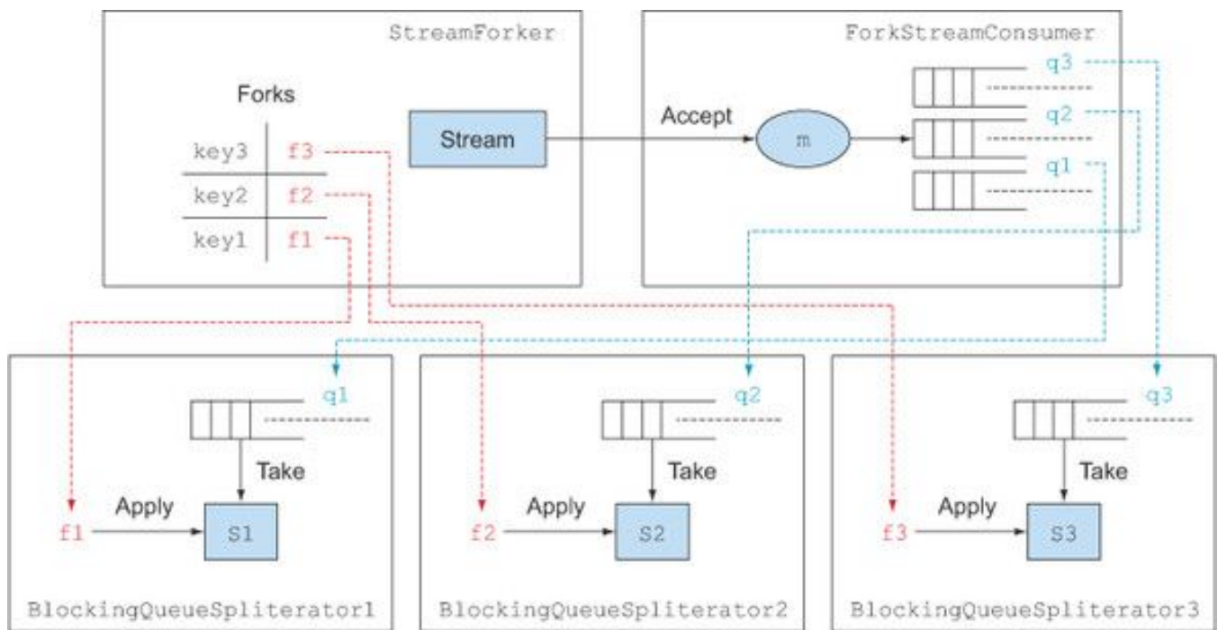
Figure C.2. The StreamForker building blocks
