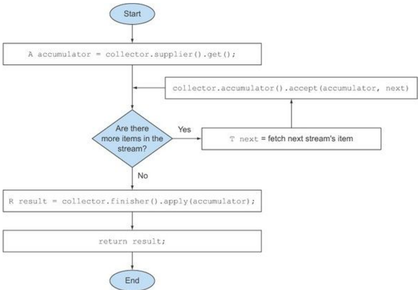
Figure 6.7. Logical steps of the sequential reduction process
