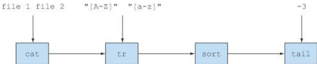
Figure 1.2. Unix commands operating on streams
