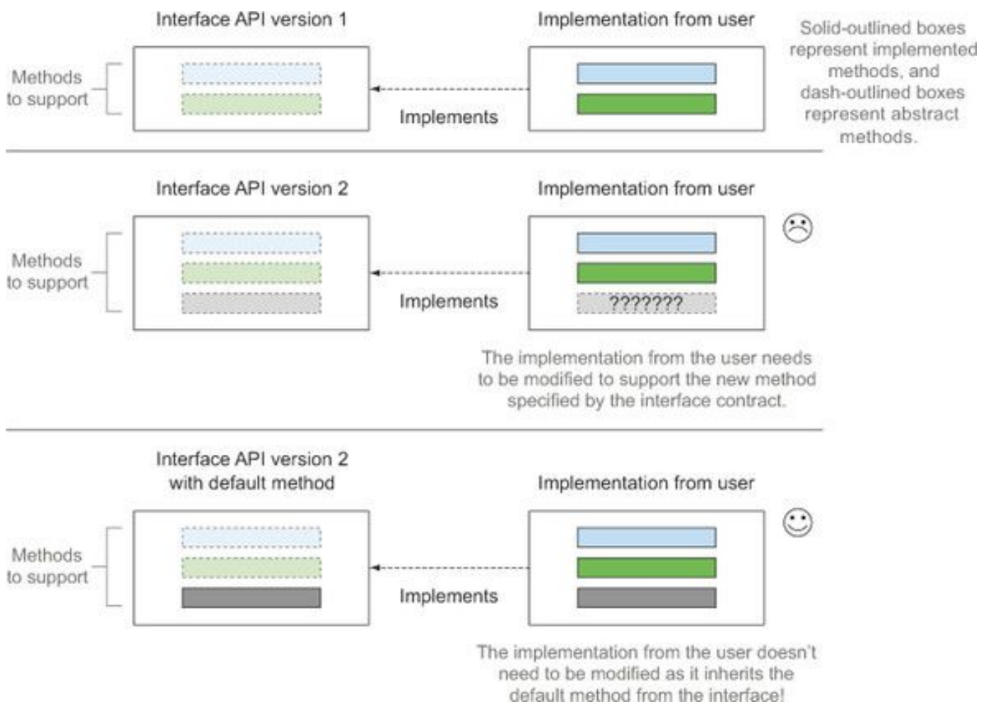
Figure 9.1. Adding a method to an interface
