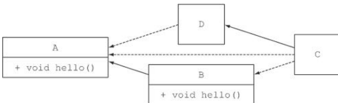
Figure 9.6. Inheriting from a class and implementing two interfaces
