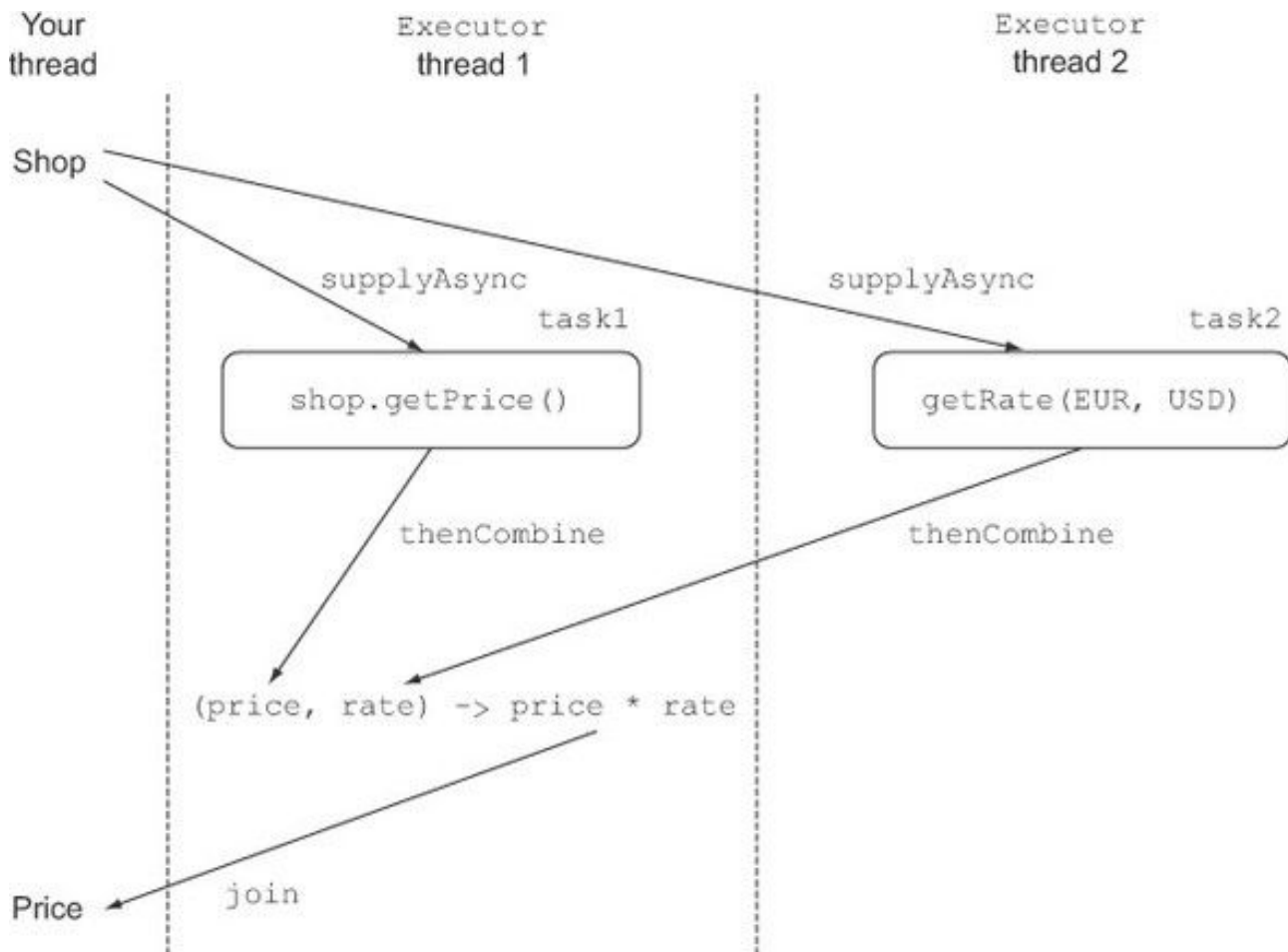
Figure 11.6. Combining two independent asynchronous tasks
