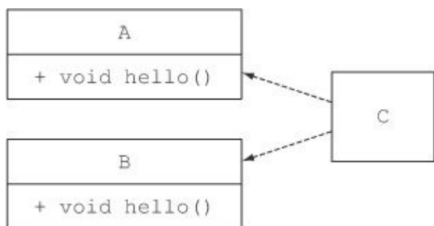
Figure 9.7. Implementing two interfaces
