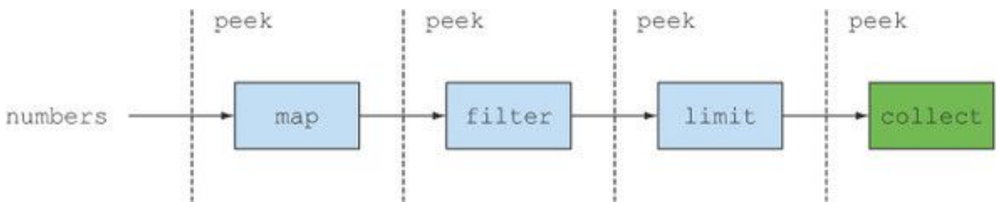
Figure 8.4. Examining values flowing in a stream pipeline with peek
