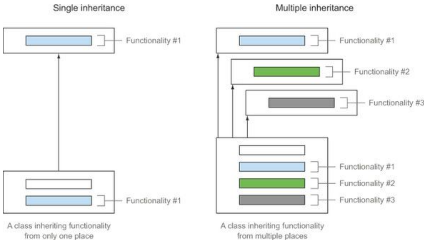
Figure 9.3. Single inheritance vs. multiple inheritance
