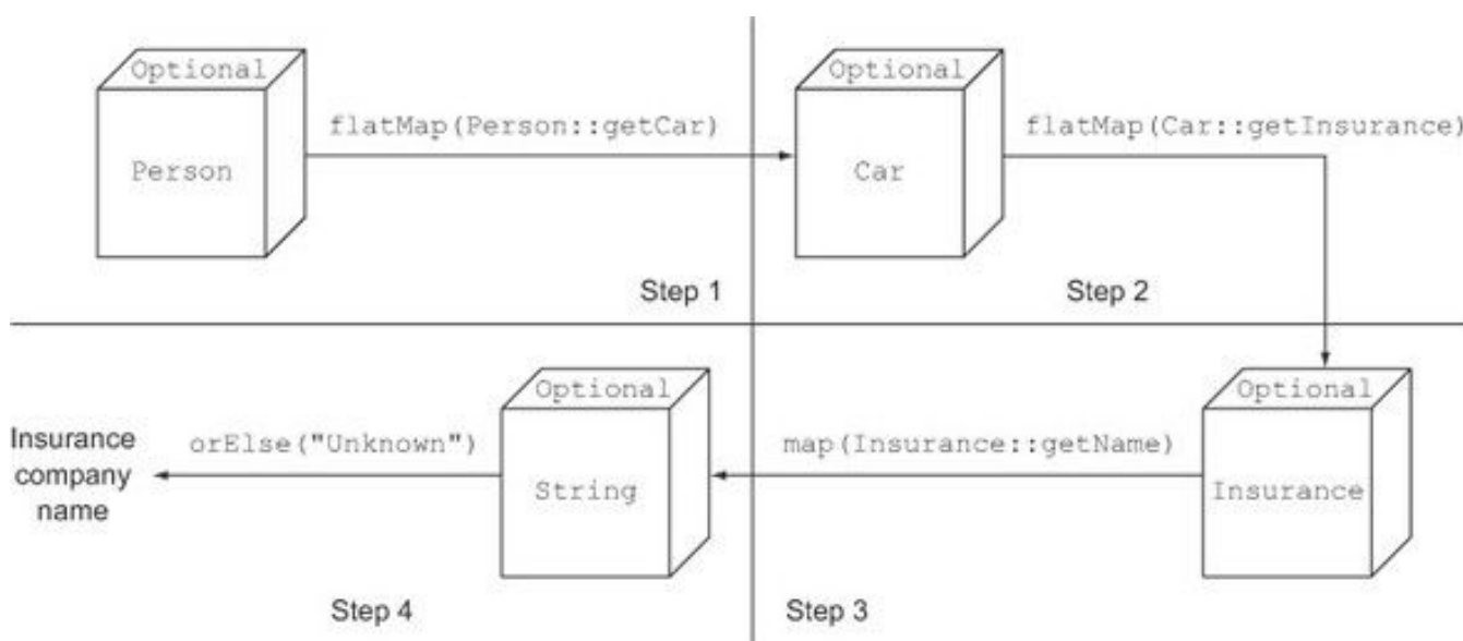
Figure 10.5. The Person/Car/Insurance dereferencing chain using optionals
