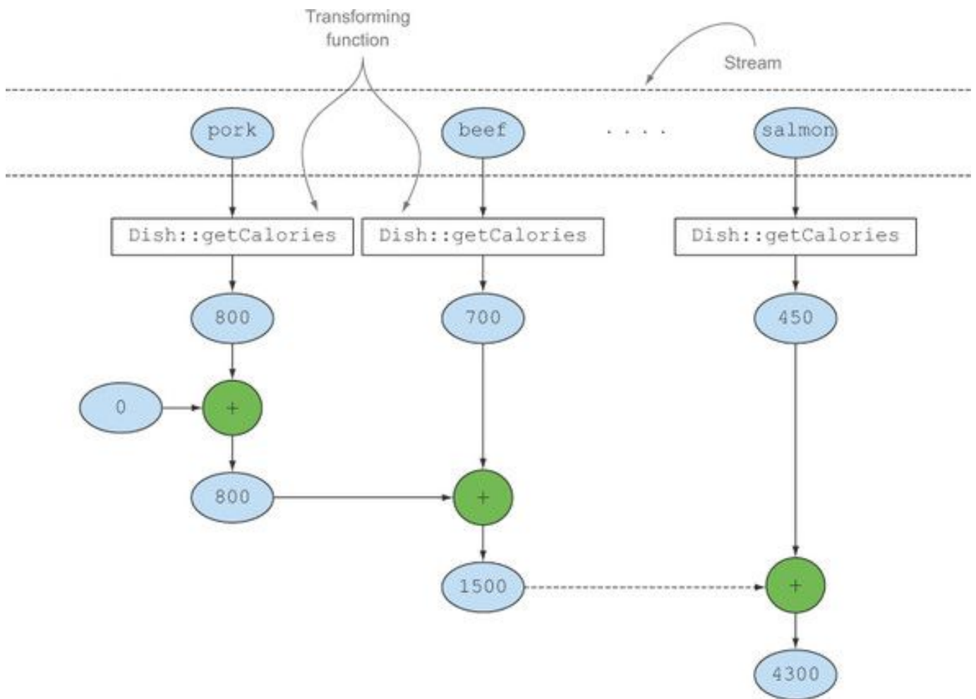
Figure 6.2. The aggregation process of the summingInt collector
