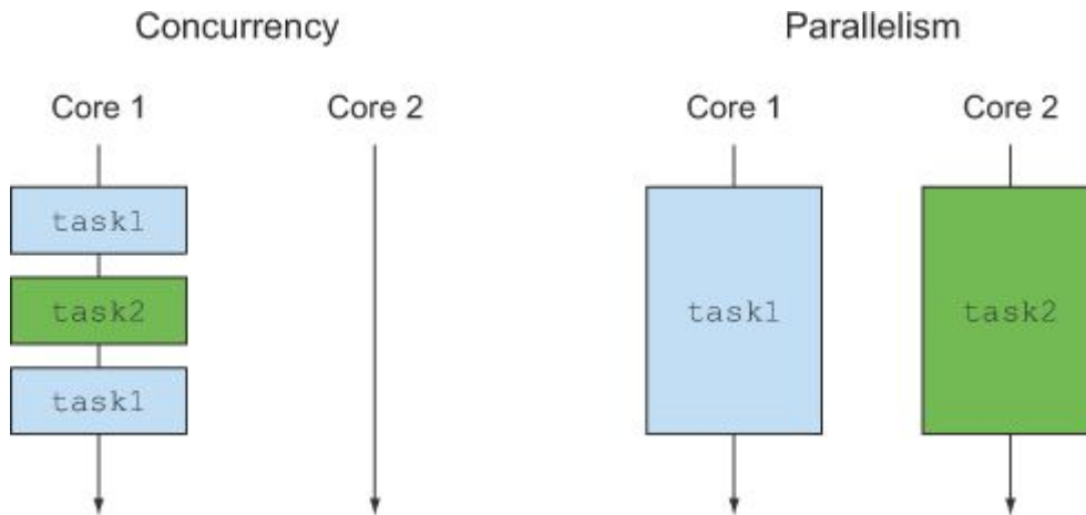
Figure 11.2. Concurrency vs. parallelism
