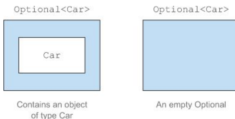
Figure 10.1. An optional Car
