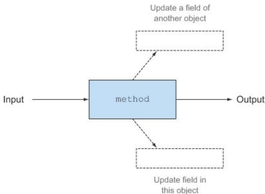
Figure 13.2. A function with side effects
