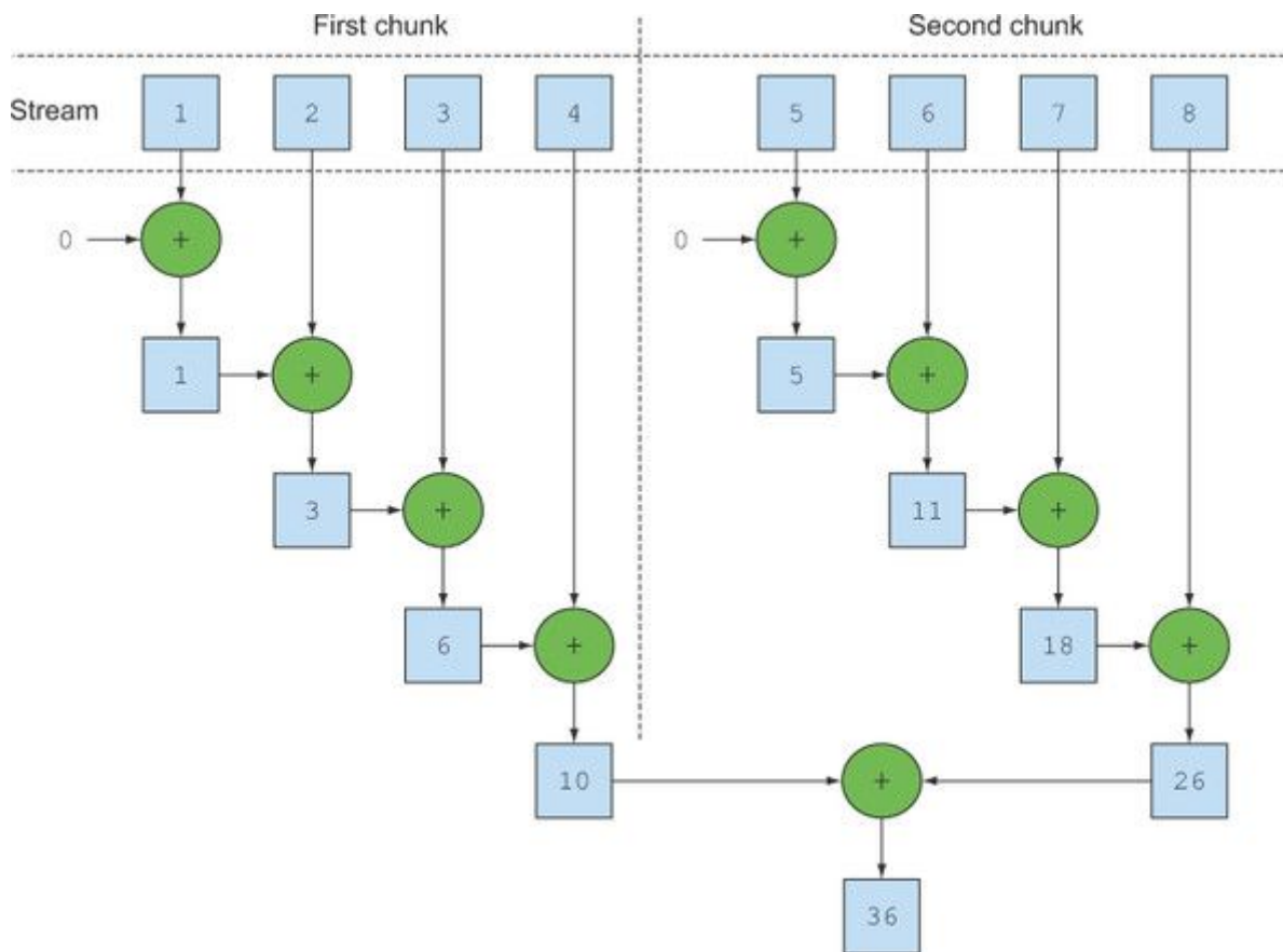
Figure 7.1. A parallel reduction operation
