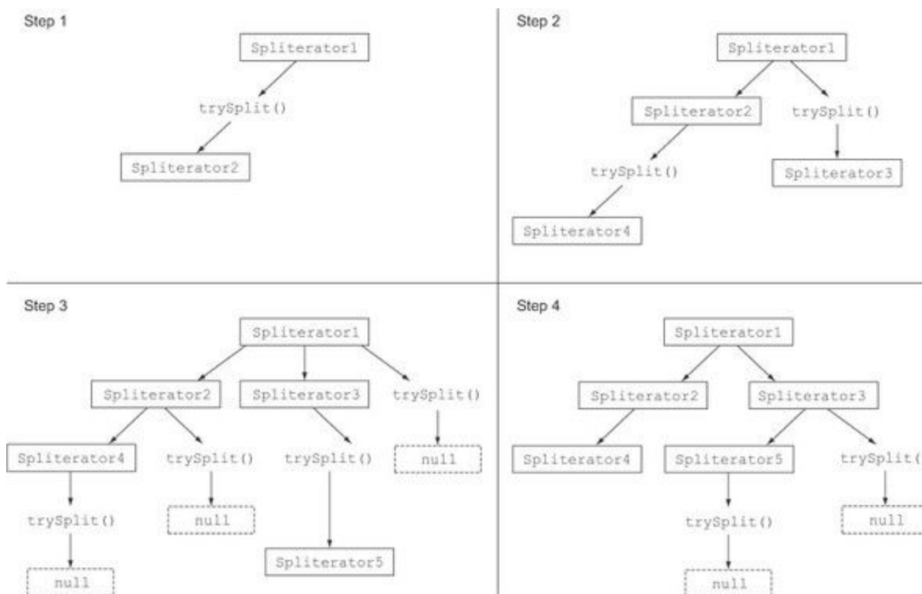
Figure 7.6. The recursive splitting process
