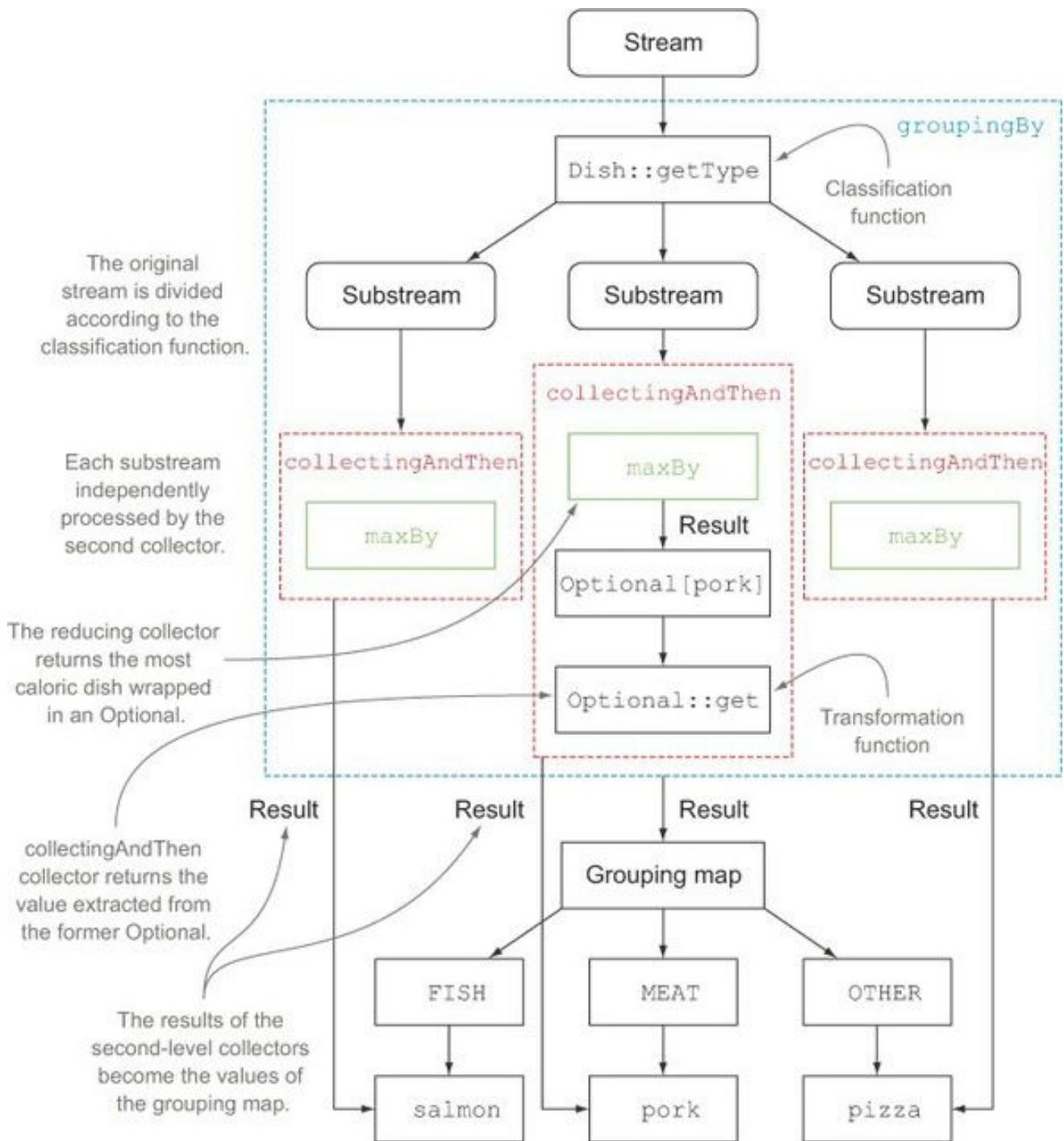
Figure 6.6. Combining the effect of multiple collectors by nesting one inside the other
