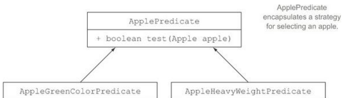
Figure 2.1. Different strategies for selecting an Apple
