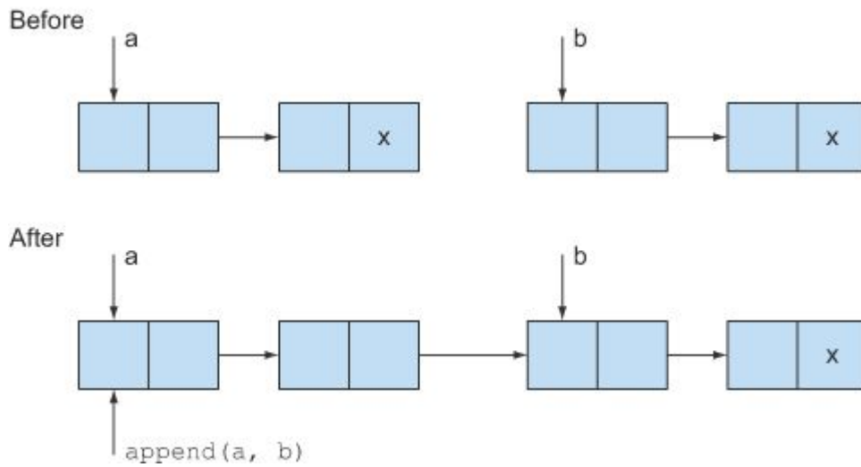
Figure 14.3. Functional style, no modifications to the data structure
