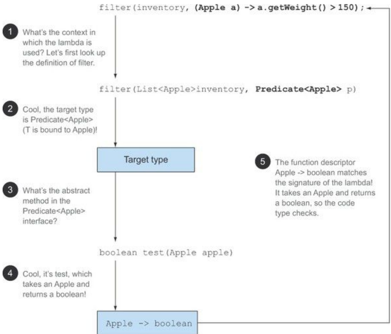
Figure 3.4. Deconstructing the type-checking process of a lambda expression
