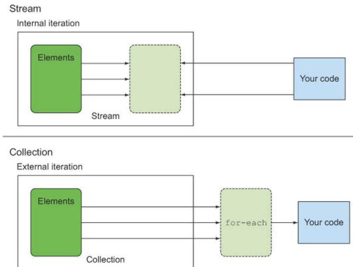
Figure 4.4. Internal vs. external iteration
