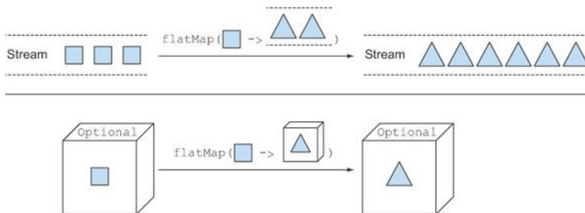
Figure 10.4. Comparing the flatMap methods of Stream and Optional
