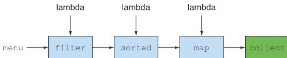
Figure 4.1. Chaining stream operations forming a stream pipeline
