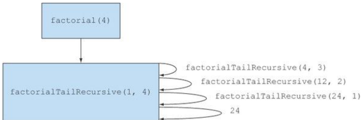
Figure 13.6. Tail-recursive definition of factorial, which can reuse a single stack frame
