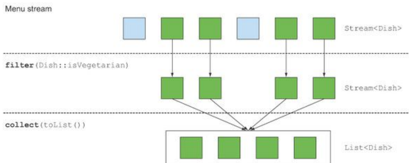
Figure 5.1. Filtering a stream with a predicate
